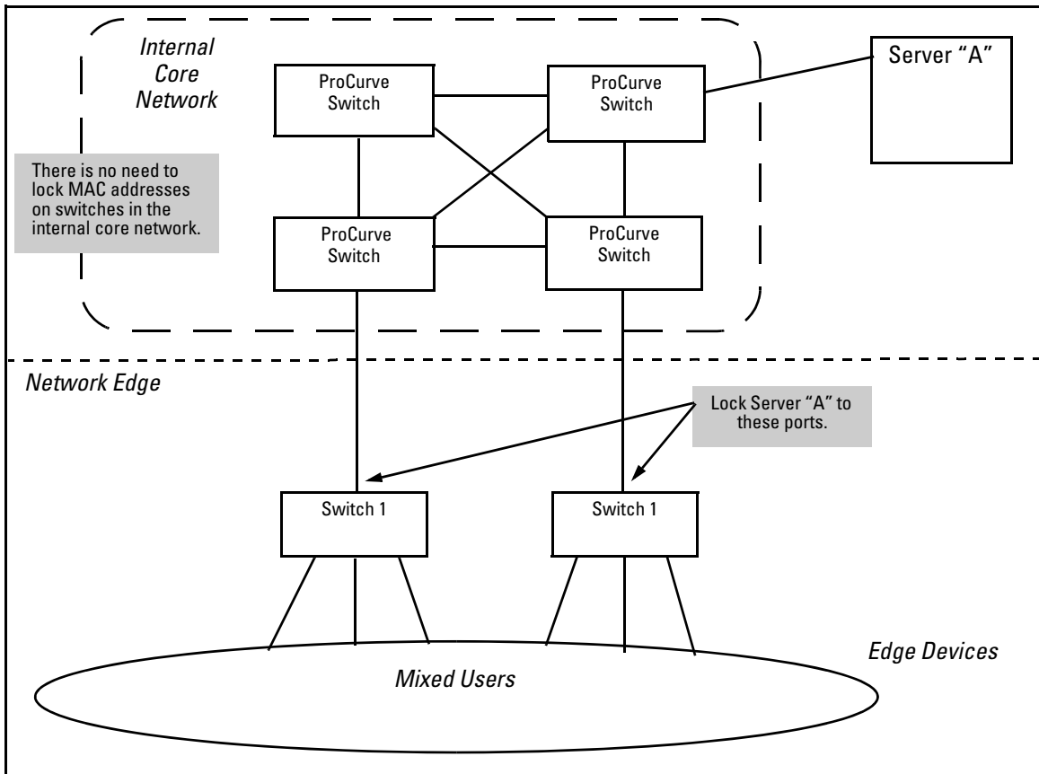
Figure 13-10. MAC Lockdown Deployed At the Network Edge Provides Security
